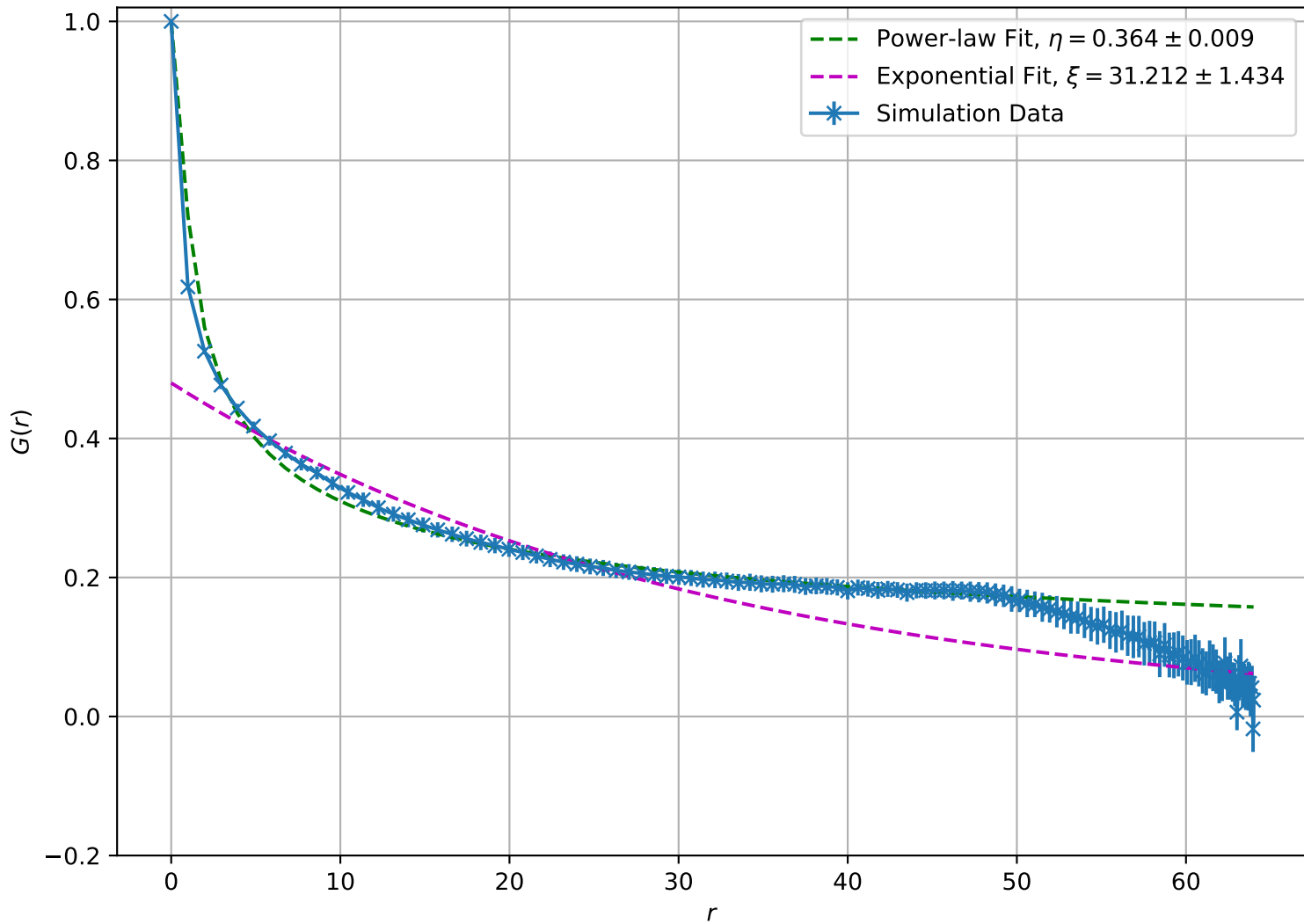
Correlation Function at T = 1.50\text{e} + 00 , L = 64
