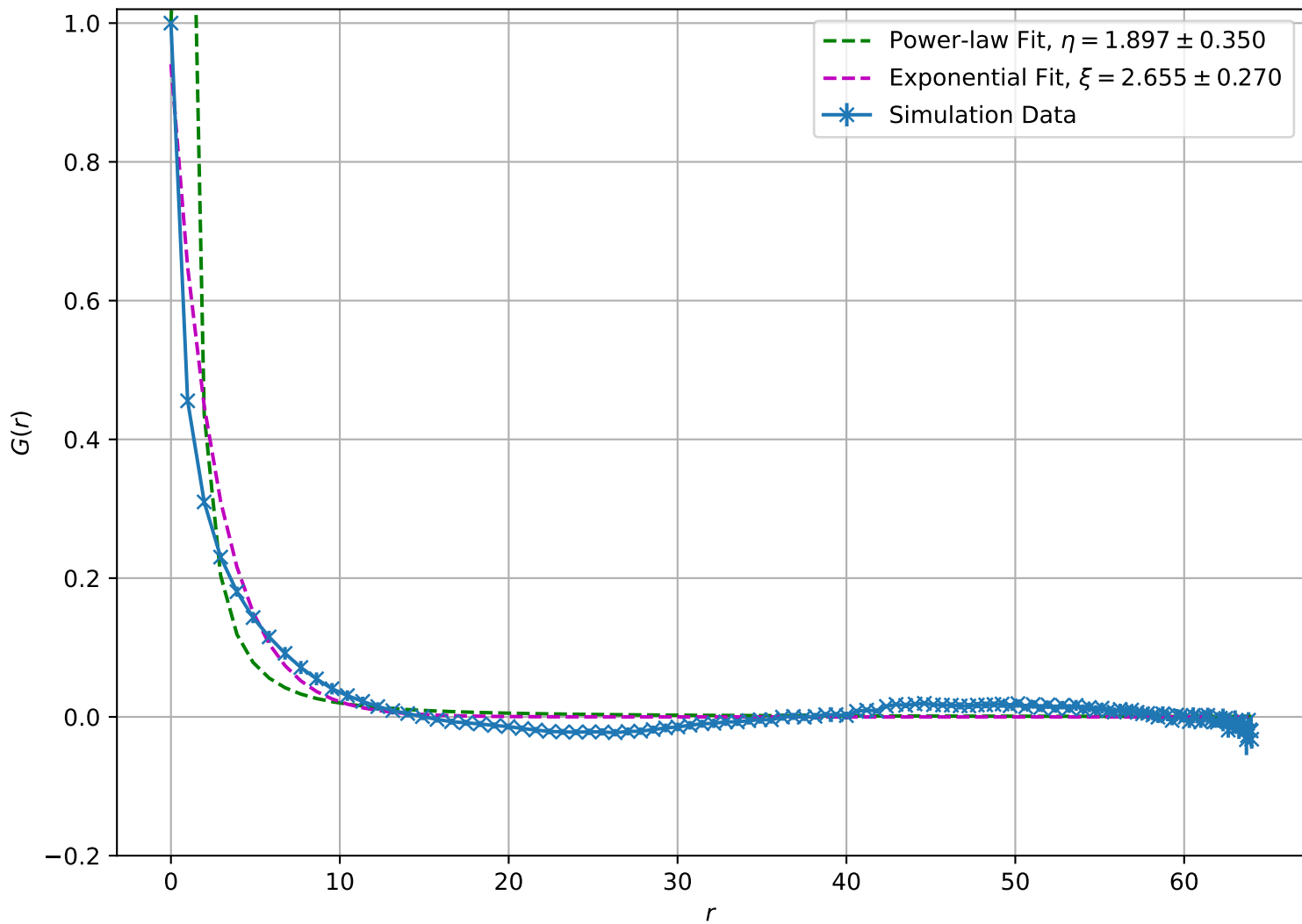
Correlation Function at T = 1.80\text{e} + 00 , L = 64
