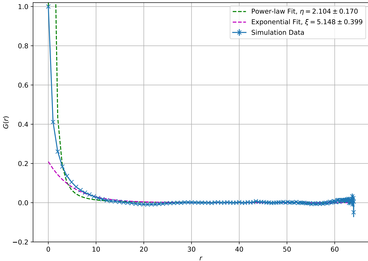
Correlation Function at T = 1.90\text{e} + 00 , L = 64
