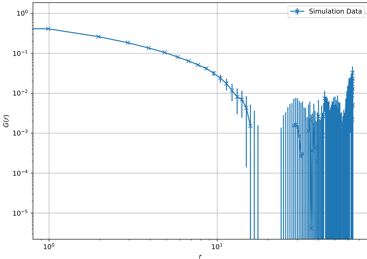
Correlation Function at T = 1.90e + 00 , L = 64 (Log-Log Scale)
