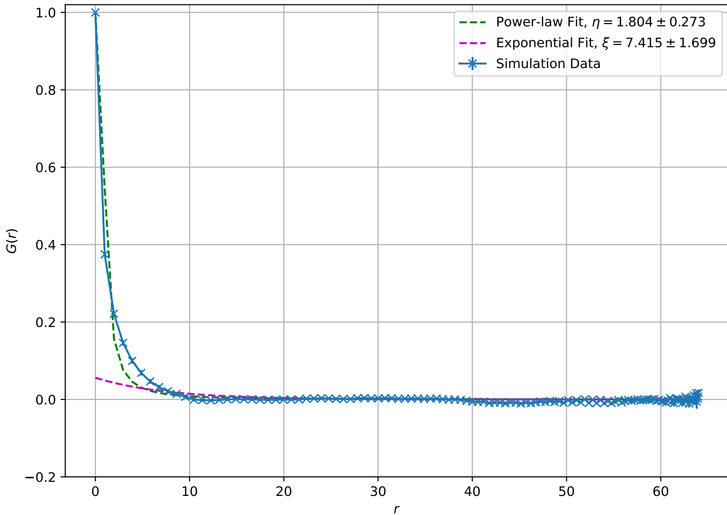
Correlation Function at T = 2.00e + 00 , L = 64
