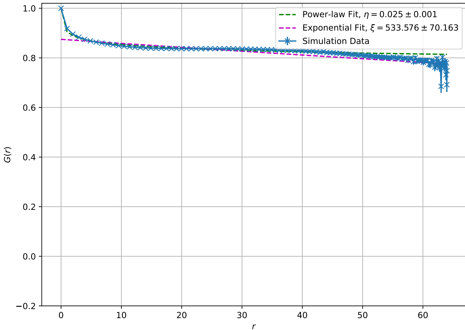
Correlation Function at T = 4.00\text{e} - 01 , L = 64
