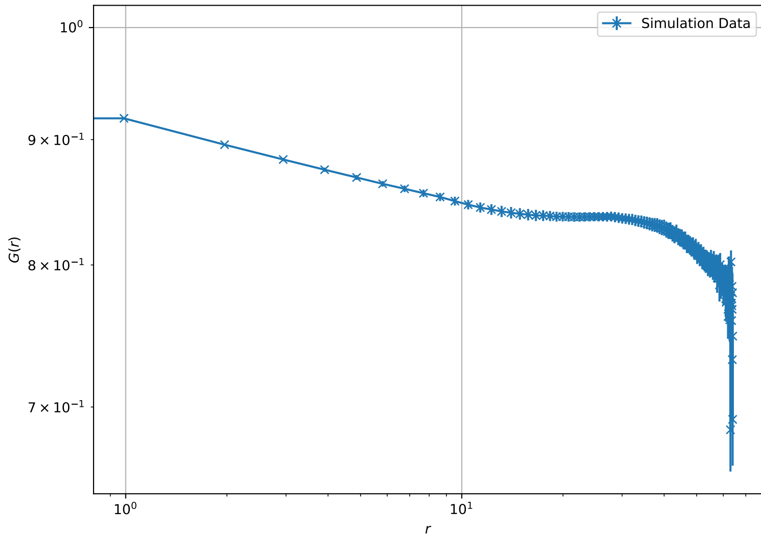
Correlation Function at T = 4.00e - 01 , L = 64 (Log-Log Scale)
