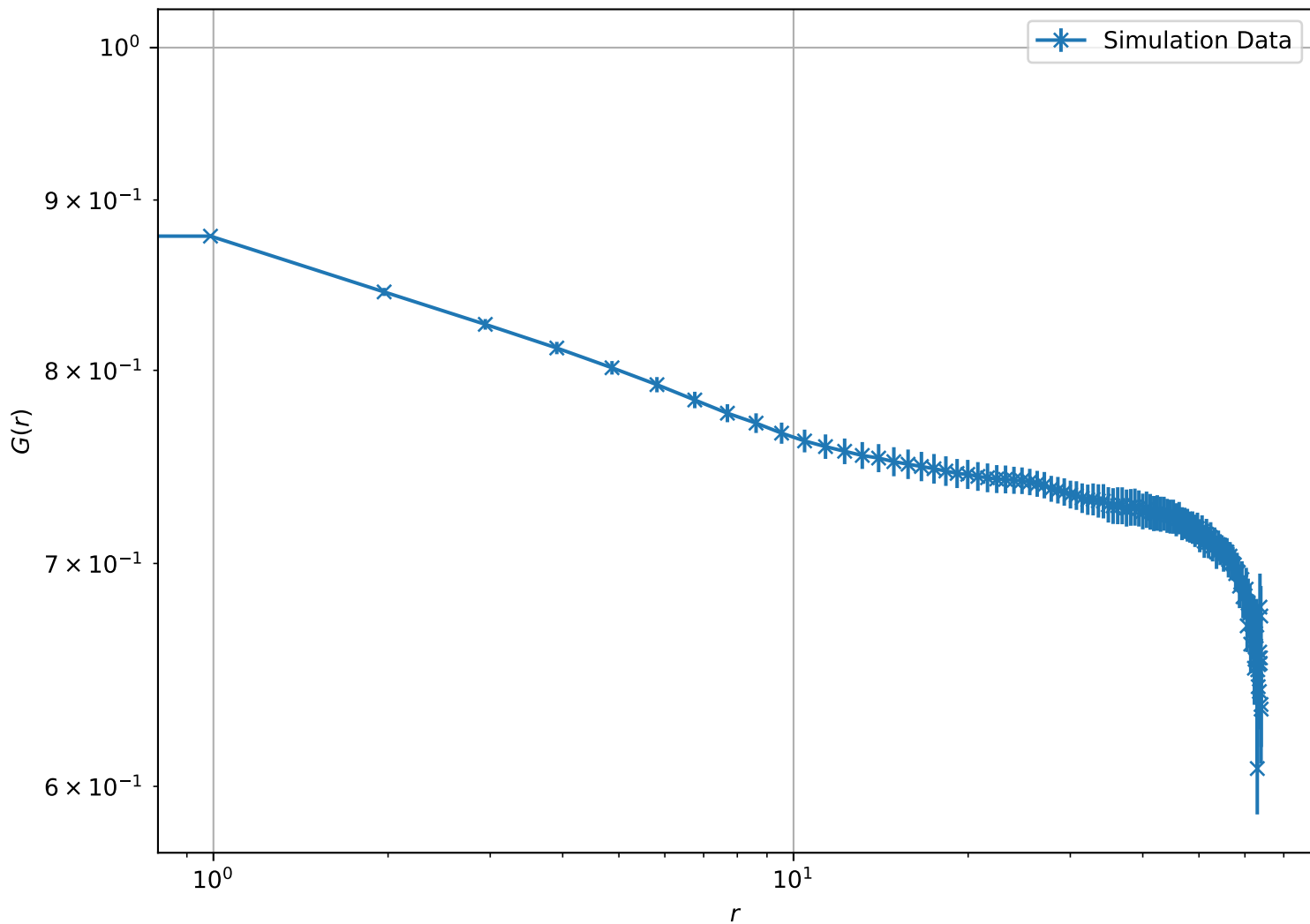
Correlation Function at T = 6.00e - 01 , L = 64 (Log-Log Scale)
