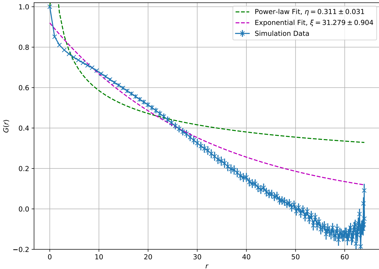
Correlation Function at T = 7.00\text{e} - 01 , L = 64
