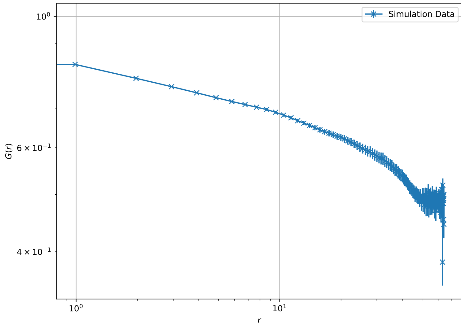
Correlation Function at T = 8.00\text{e} - 01 , L = 64 (Log-Log Scale)
