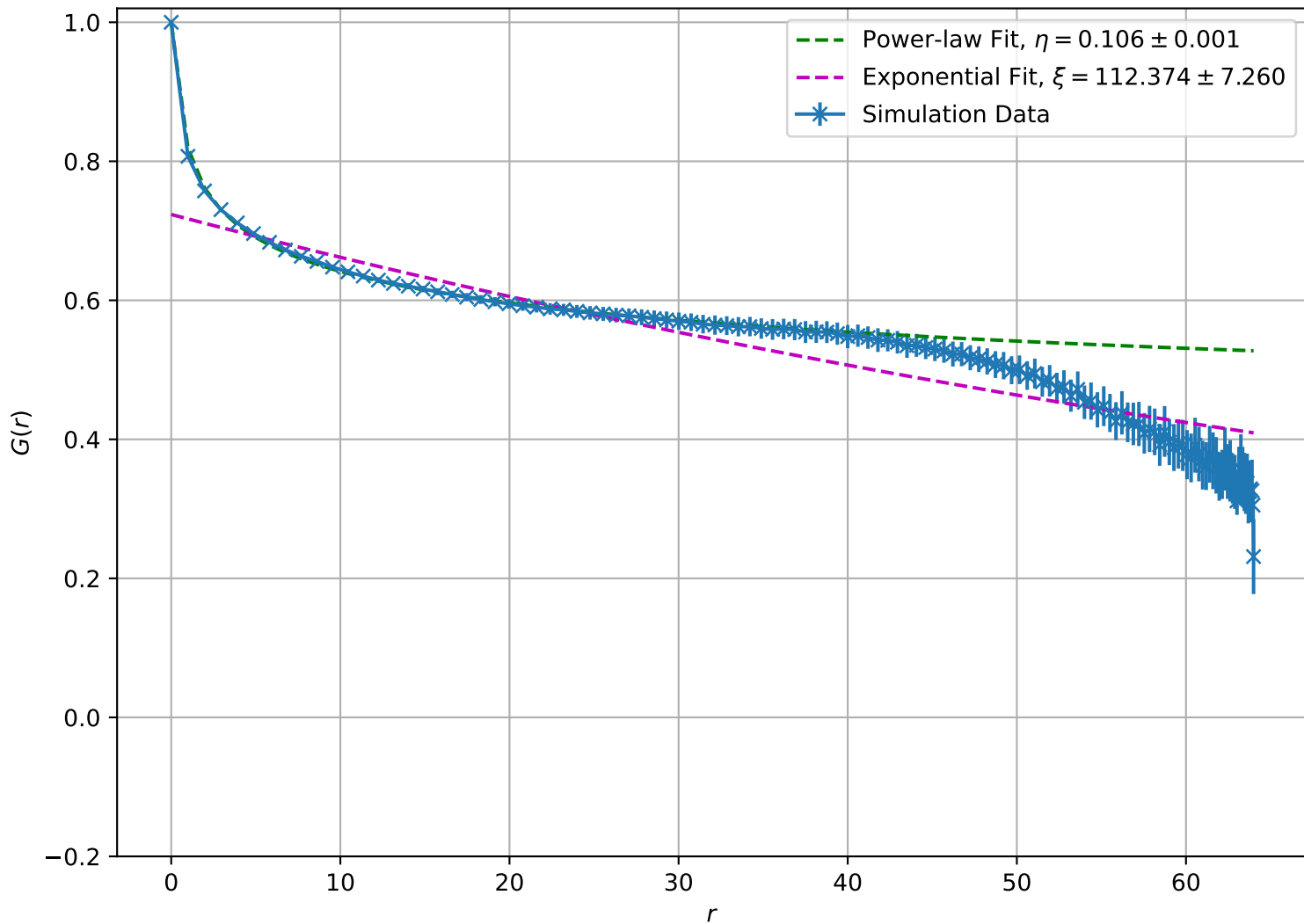
Correlation Function at T = 9.00\text{e} - 01 , L = 64
