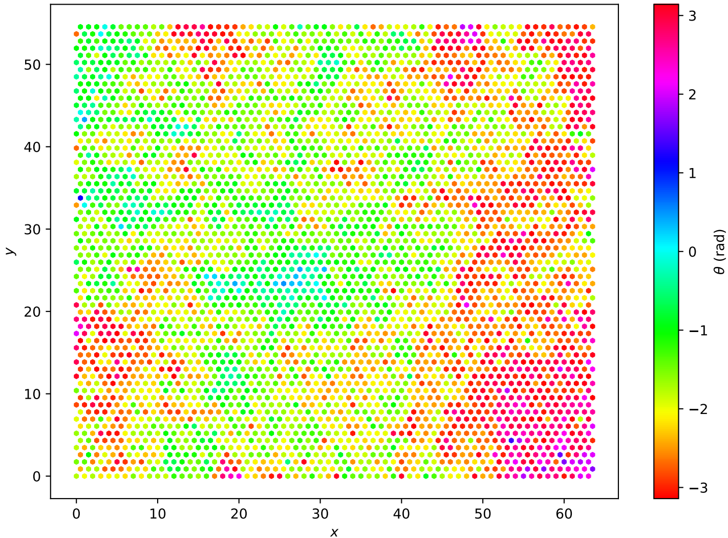
Hexagonal Lattice L=64 , T = 9.00e - 01
