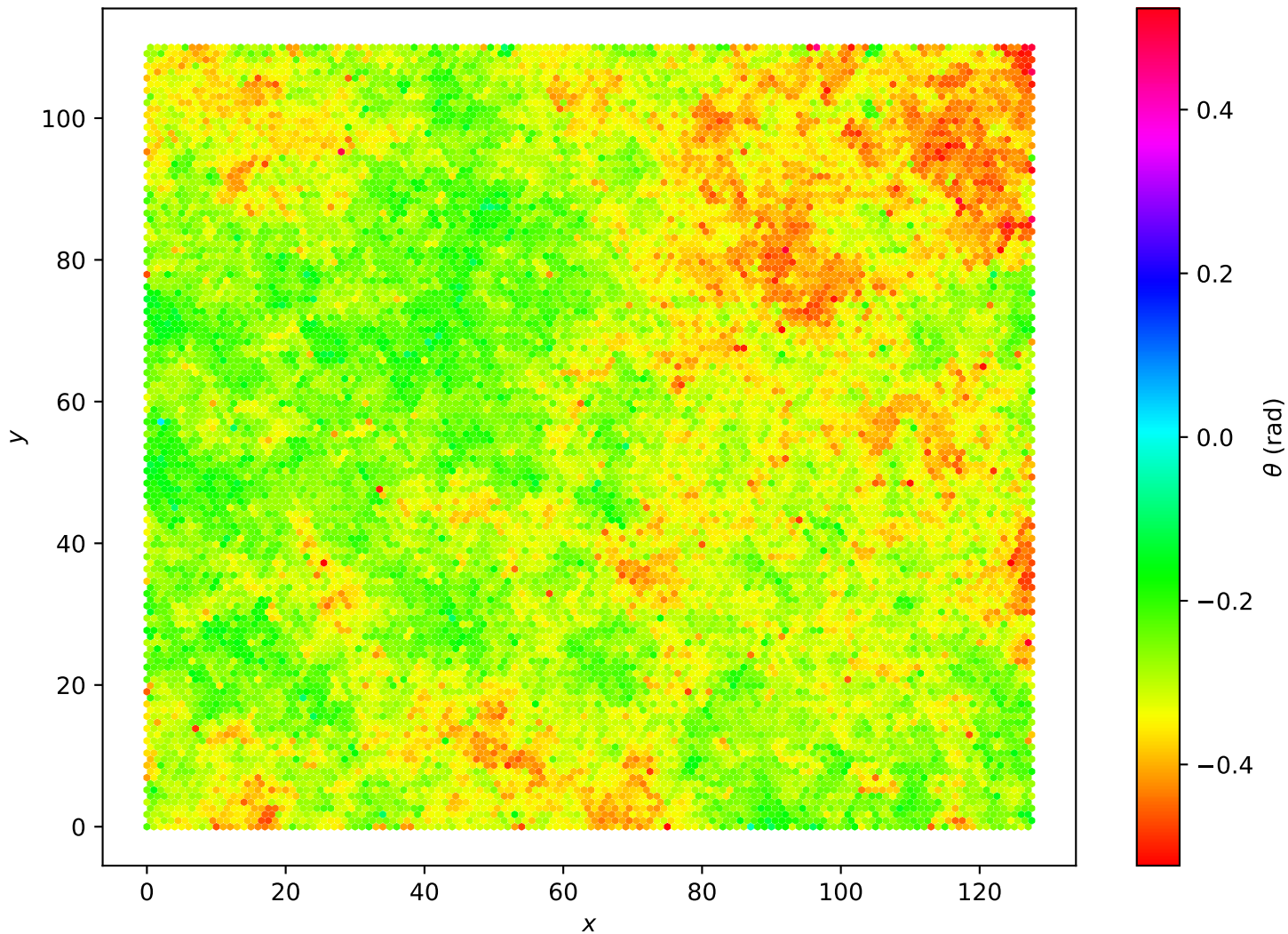
Hexagonal Lattice L=128 , T = 1.00e - 01
