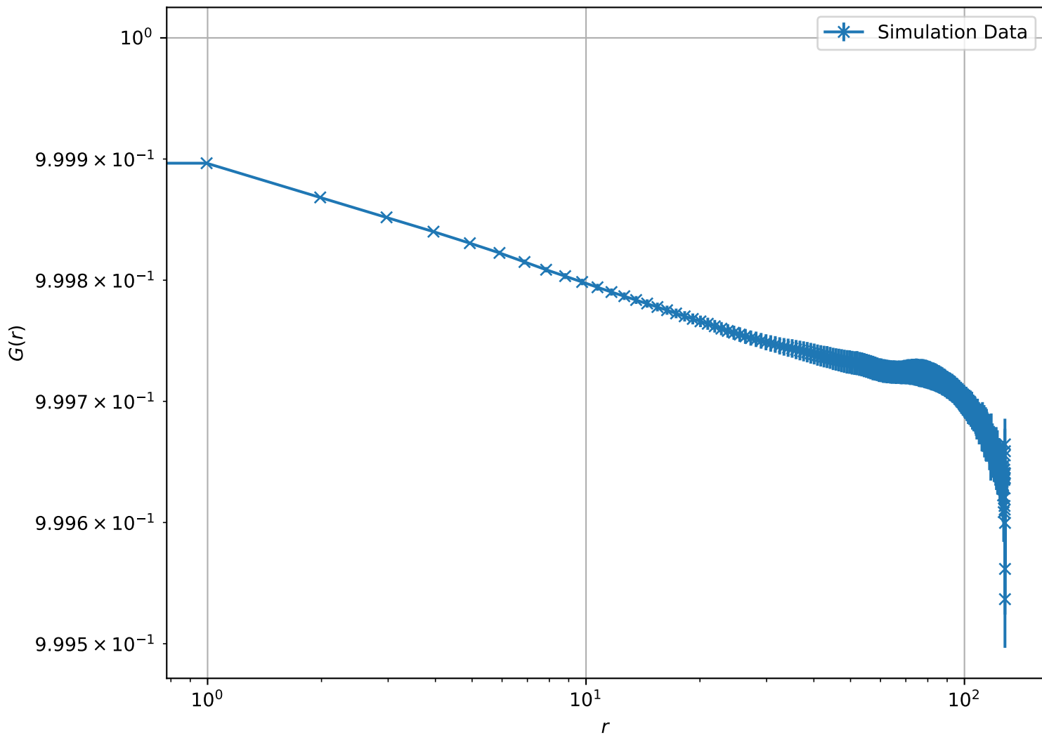
Correlation Function at T = 1.00e - 02 , L = 128 (Log-Log Scale)
