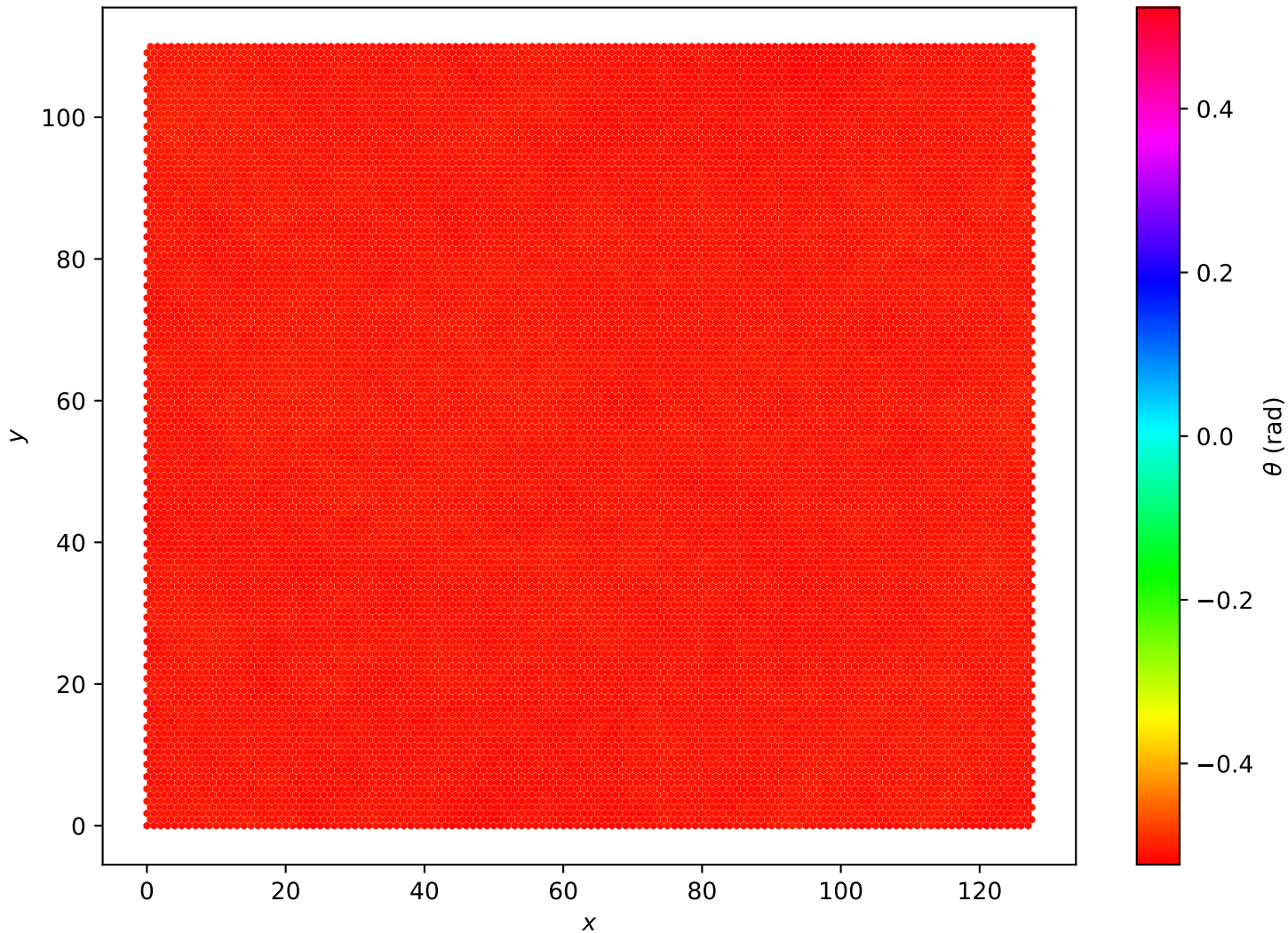
Hexagonal Lattice L=128 , T = 1.00e - 02
