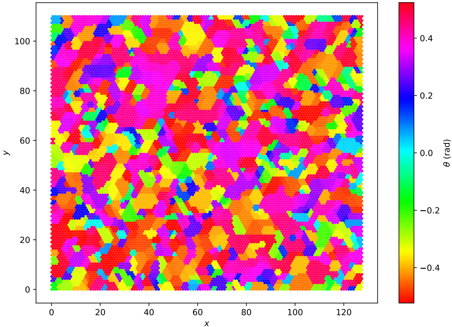
Hexagonal Lattice L=128 , T = 1.00e - 05
