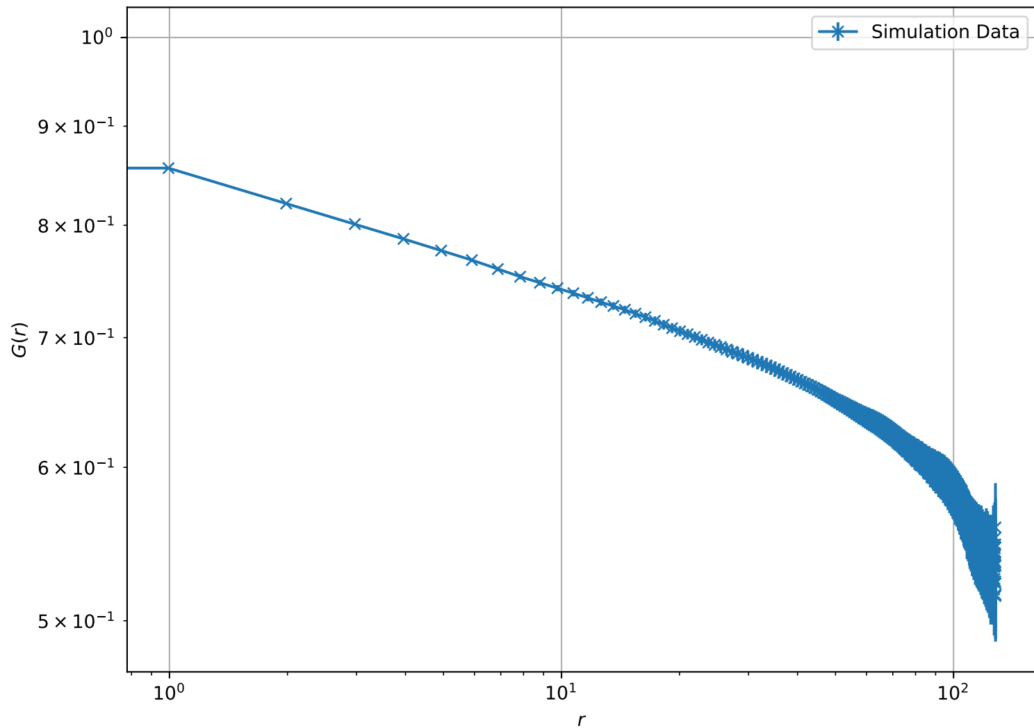
Correlation Function at T = 1.50e - 01 , L = 128 (Log-Log Scale)
