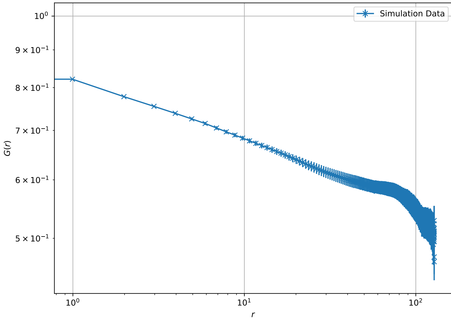
Correlation Function at T = 1.60e - 01 , L = 128 (Log-Log Scale)
