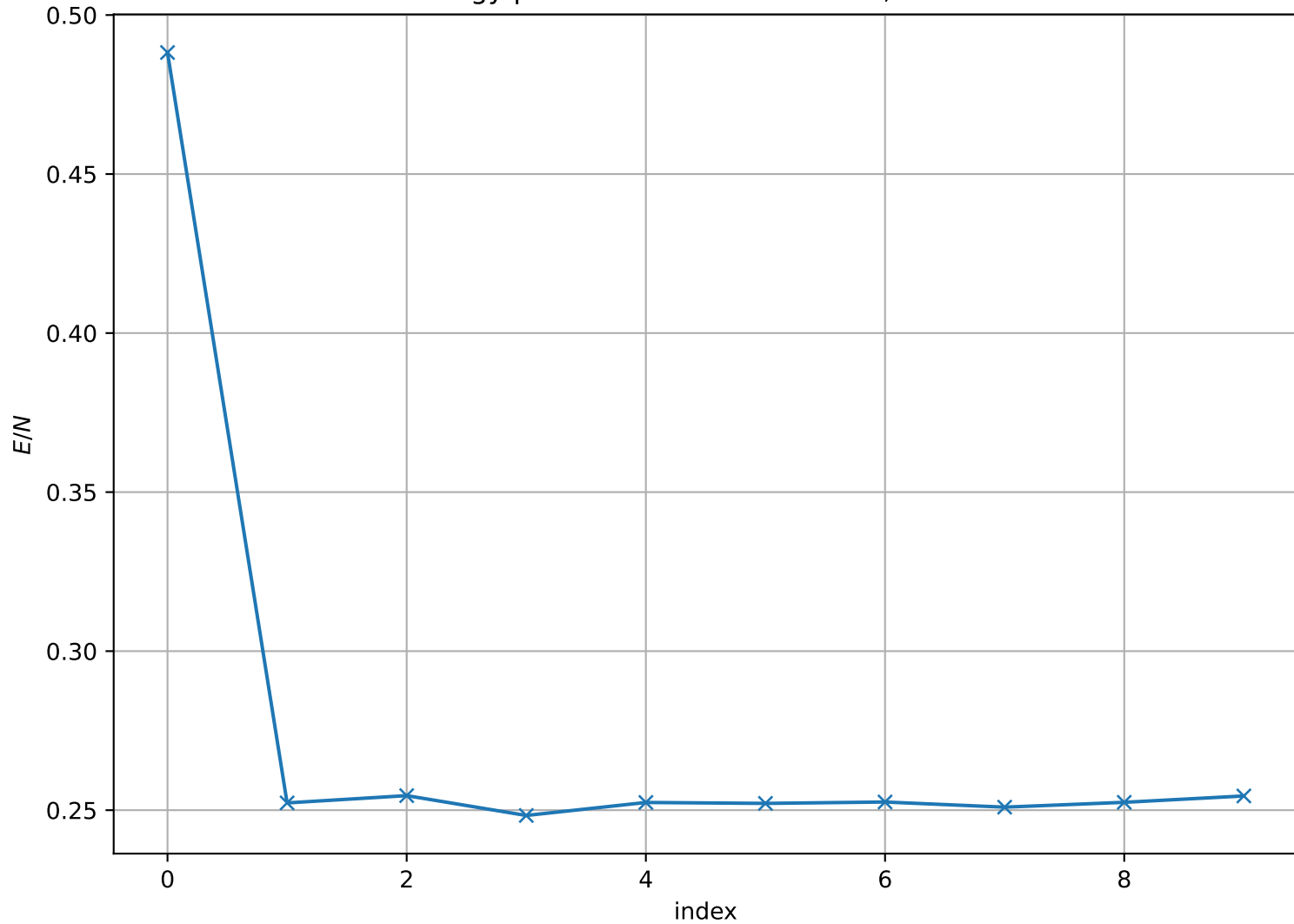
Energy per Site at T = 1.700e - 01 , L = 128
