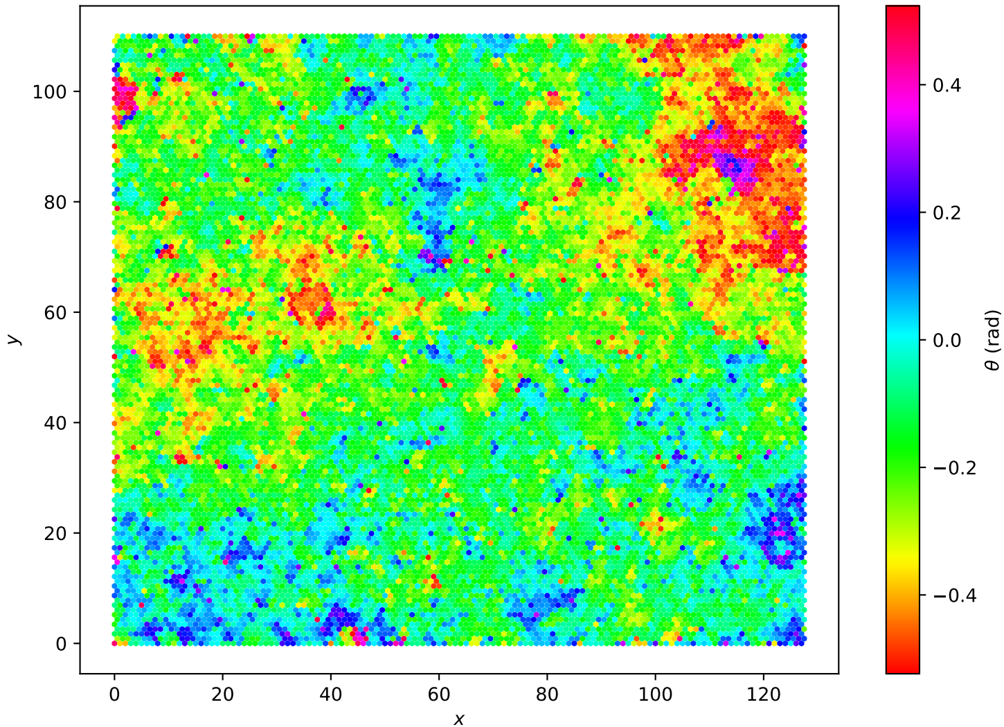
Hexagonal Lattice L=128 , T = 1.70e - 01
