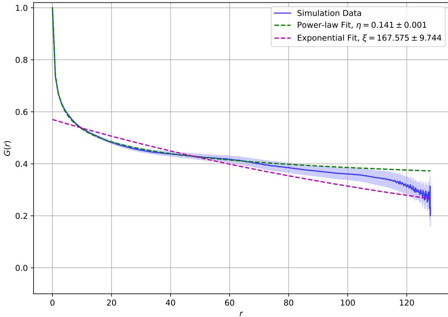
Correlation Function at T = 1.80e - 01 , L = 128
