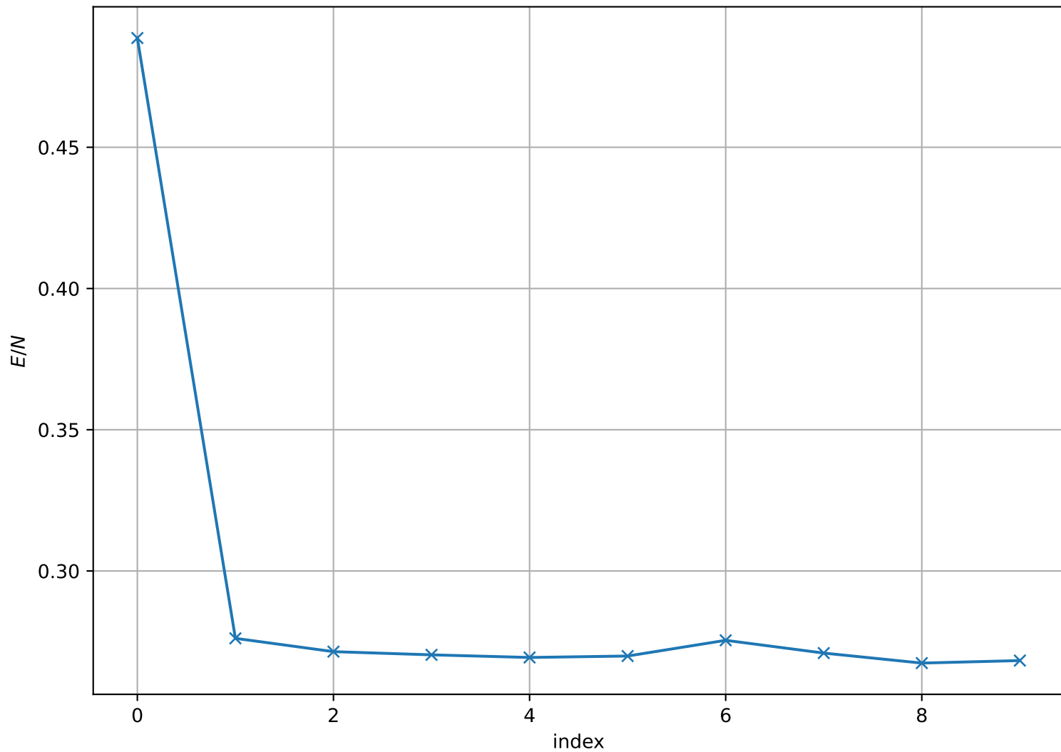
Energy per Site at T = 1.800e - 01 , L = 128
