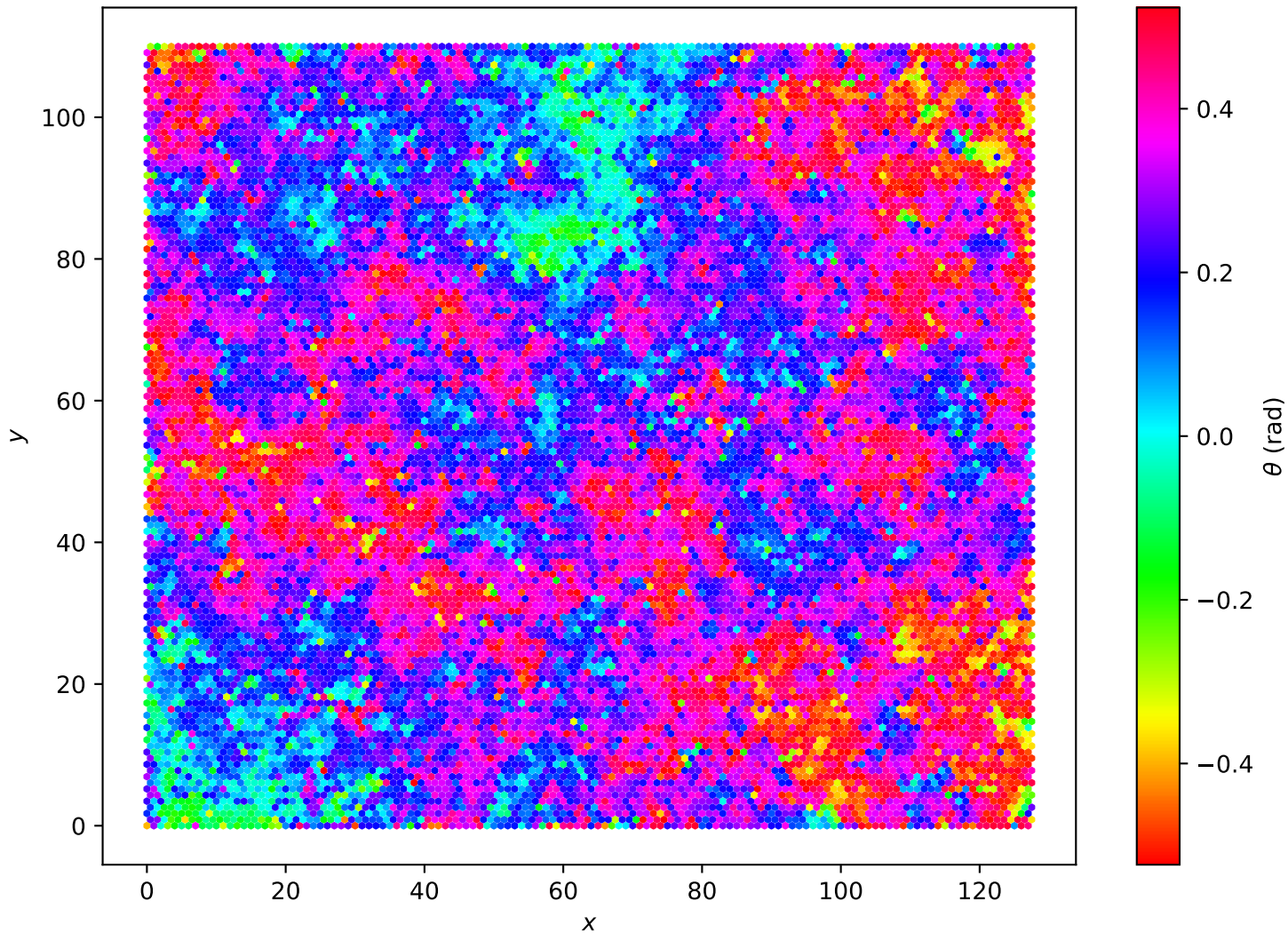
Hexagonal Lattice L=128 , T = 1.80e - 01
