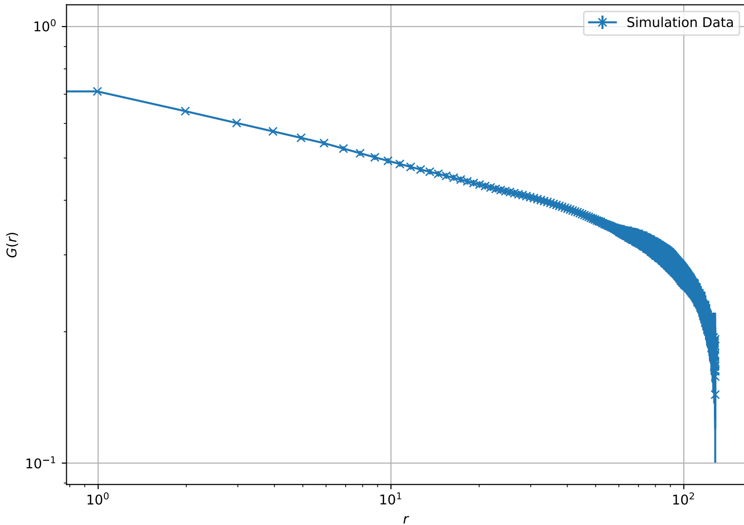
Correlation Function at T = 1.85e - 01 , L = 128 (Log-Log Scale)
