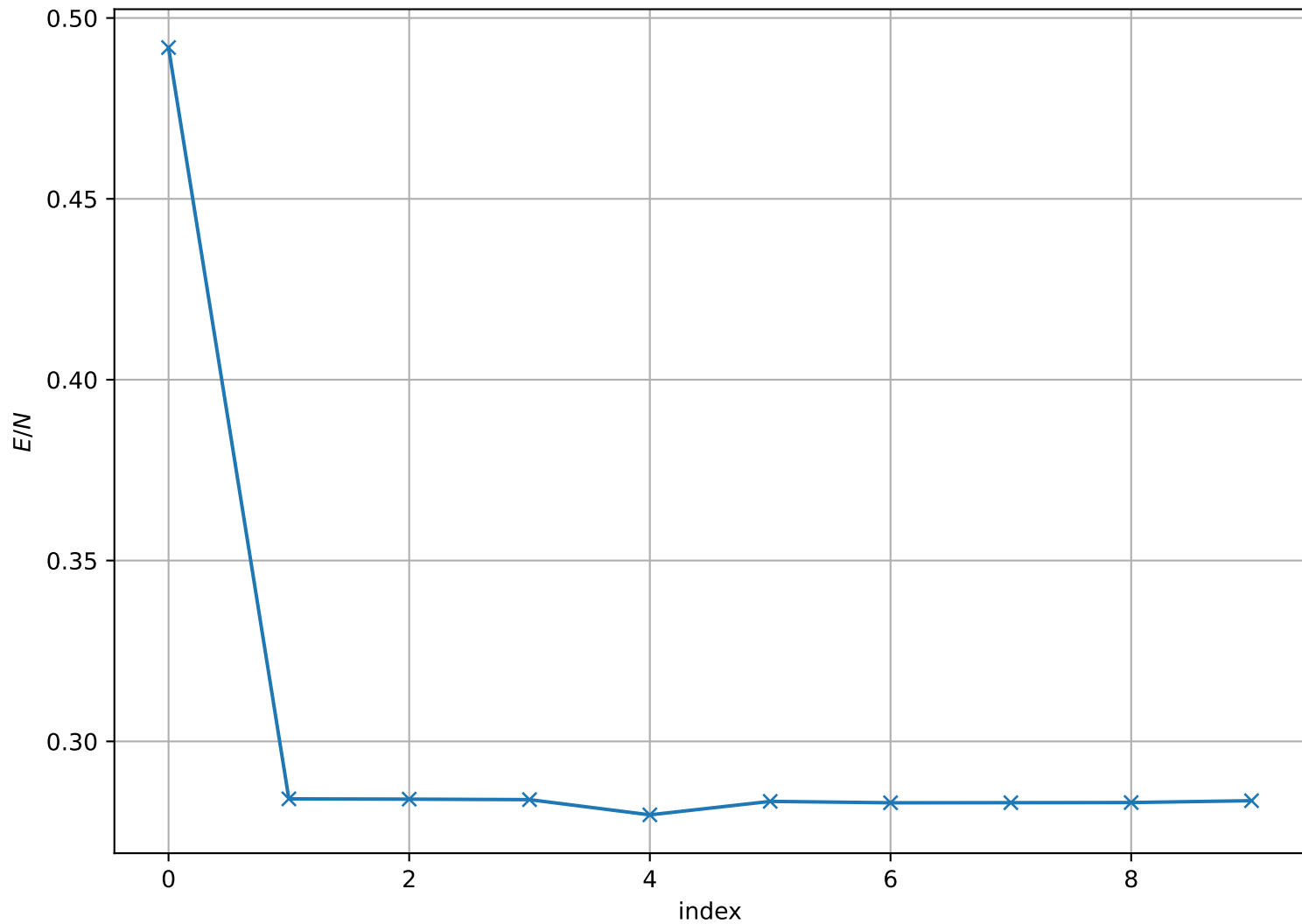
Energy per Site at T = 1.850e - 01 , L = 128
