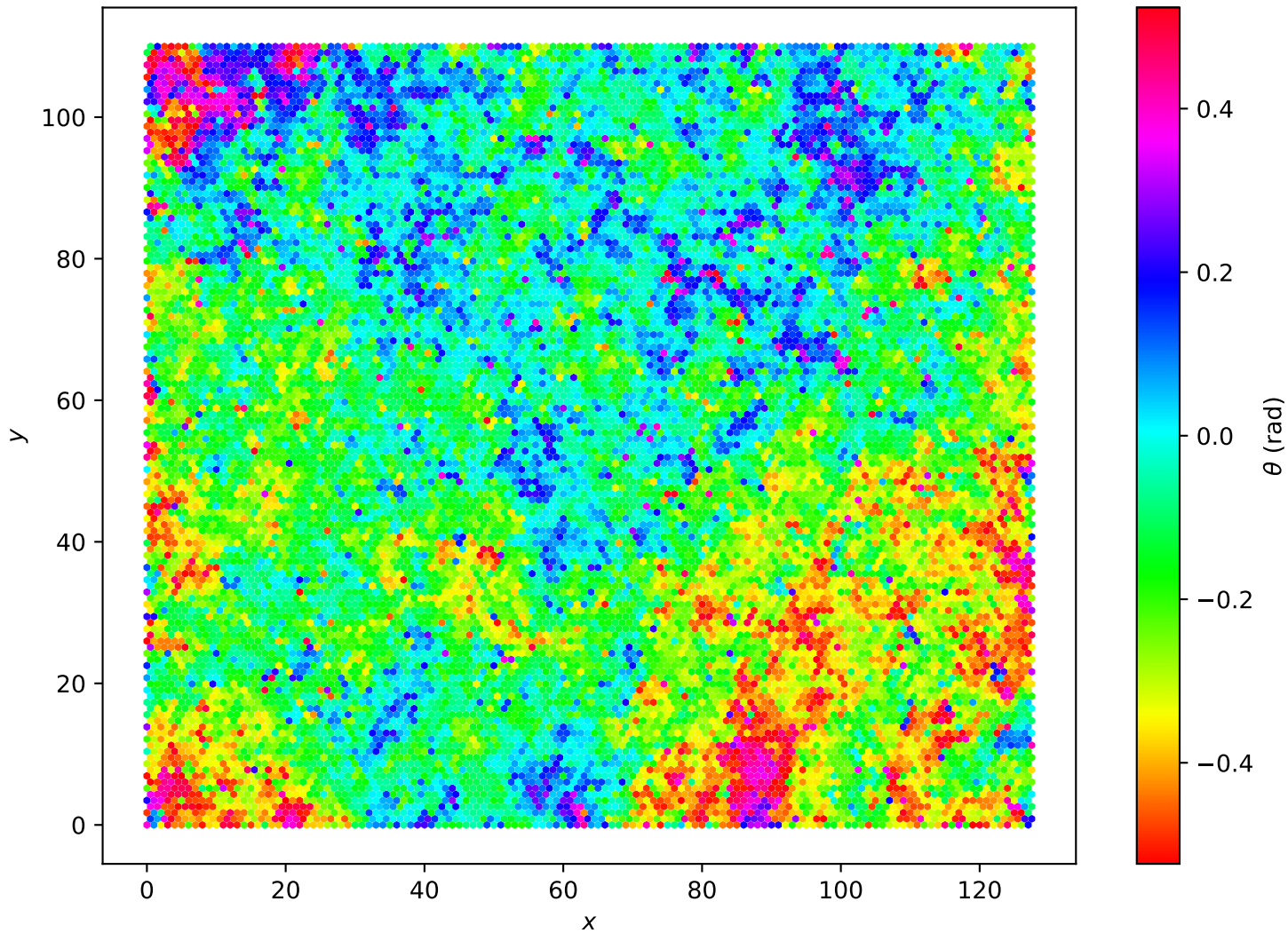
Hexagonal Lattice L=128 , T = 1.85e - 01
