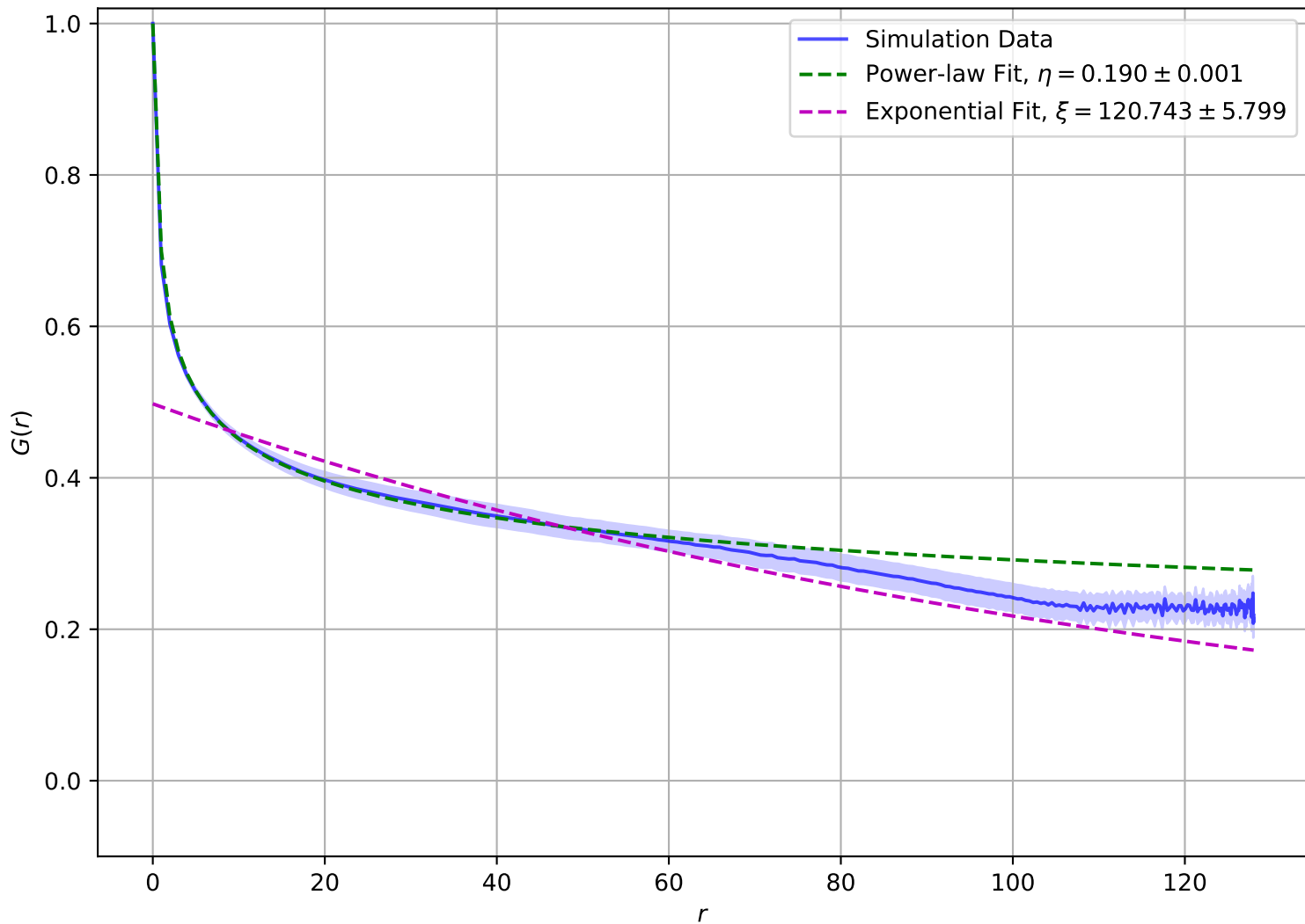
Correlation Function at T = 1.90e - 01 , L = 128
