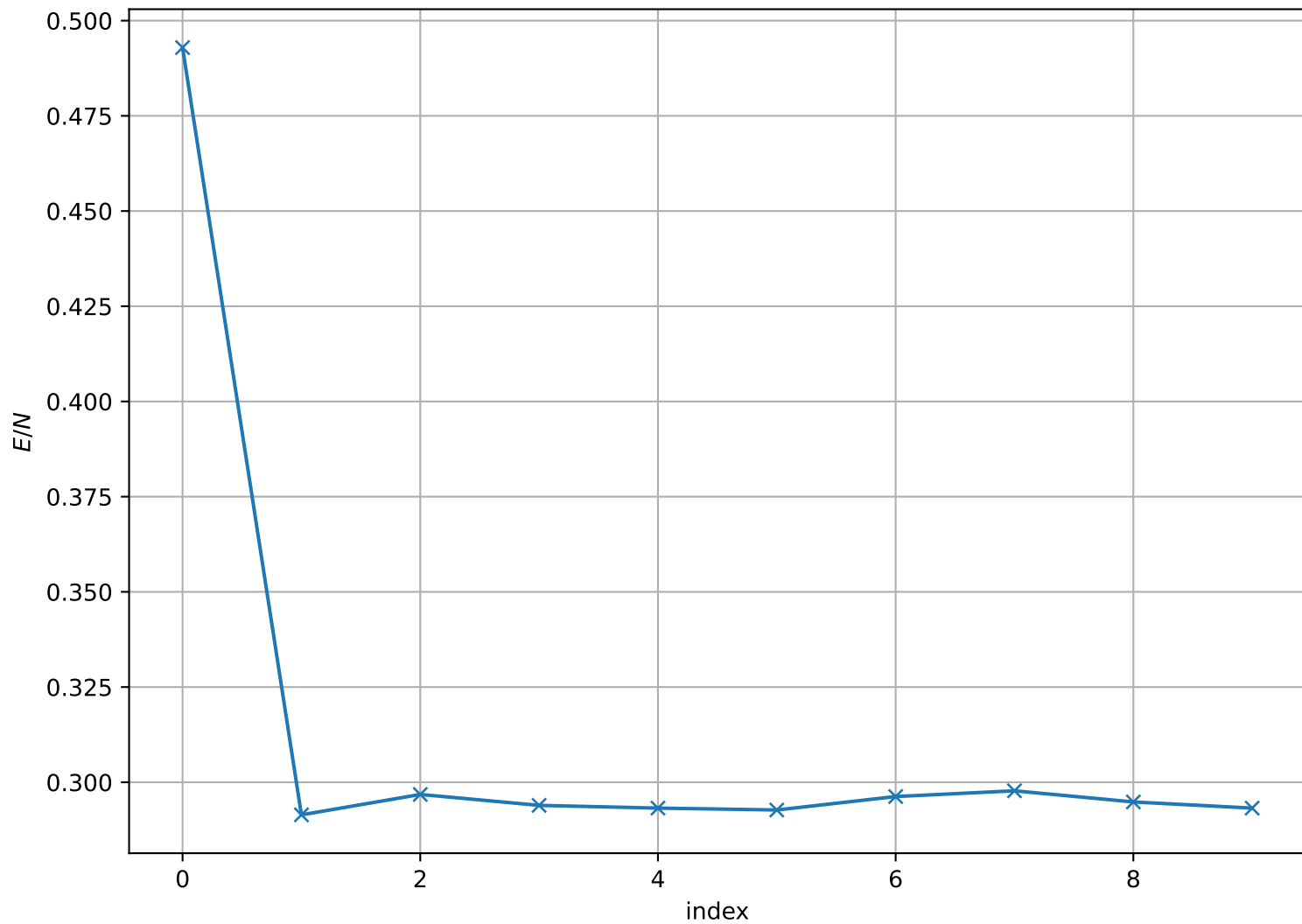
Energy per Site at T = 1.900e - 01 , L = 128
