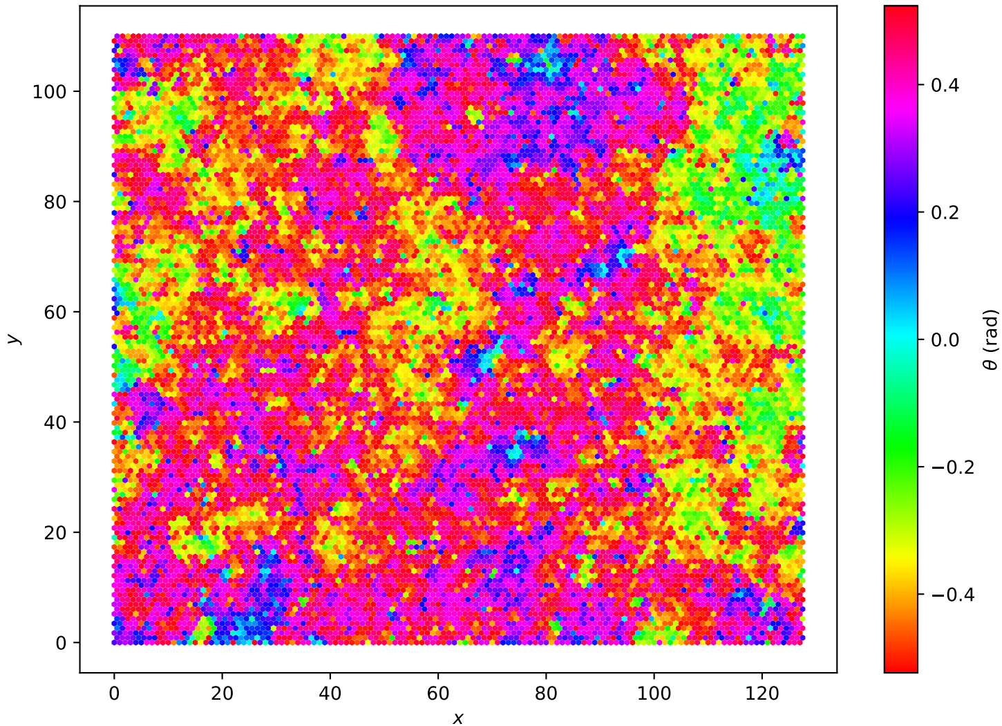
Hexagonal Lattice L=128 , T = 1.90e - 01
