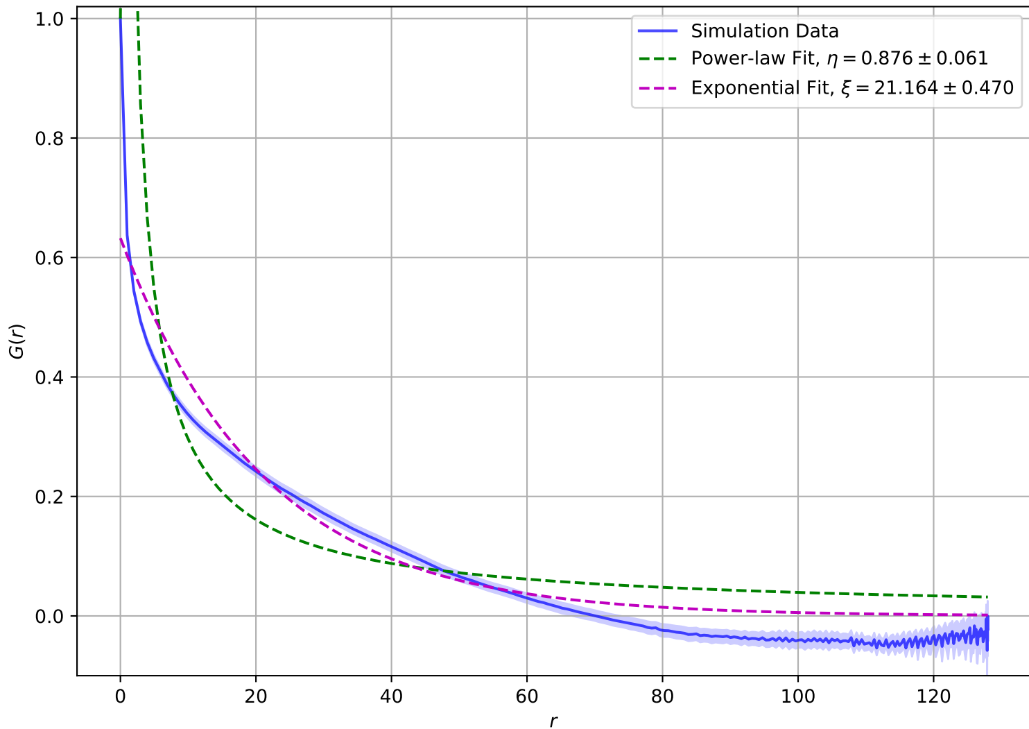
Correlation Function at T = 1.95e - 01 , L = 128
