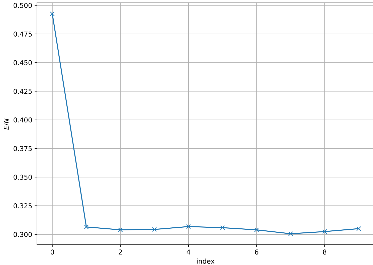
Energy per Site at T = 1.950e - 01 , L = 128
