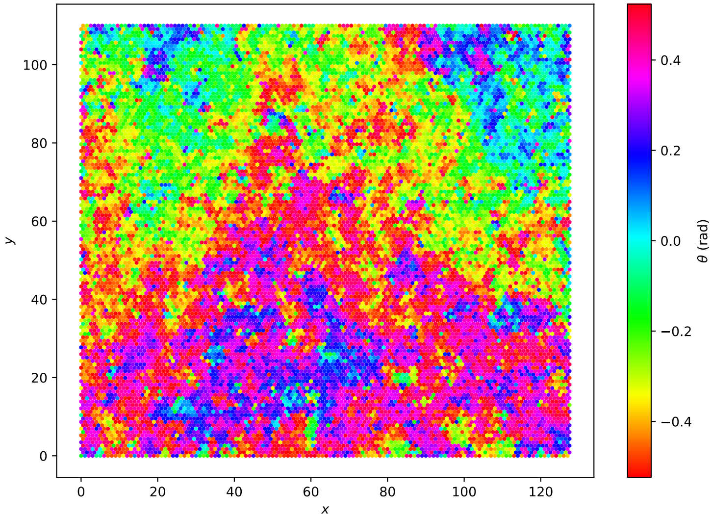
Hexagonal Lattice L=128 , T = 1.95e - 01
