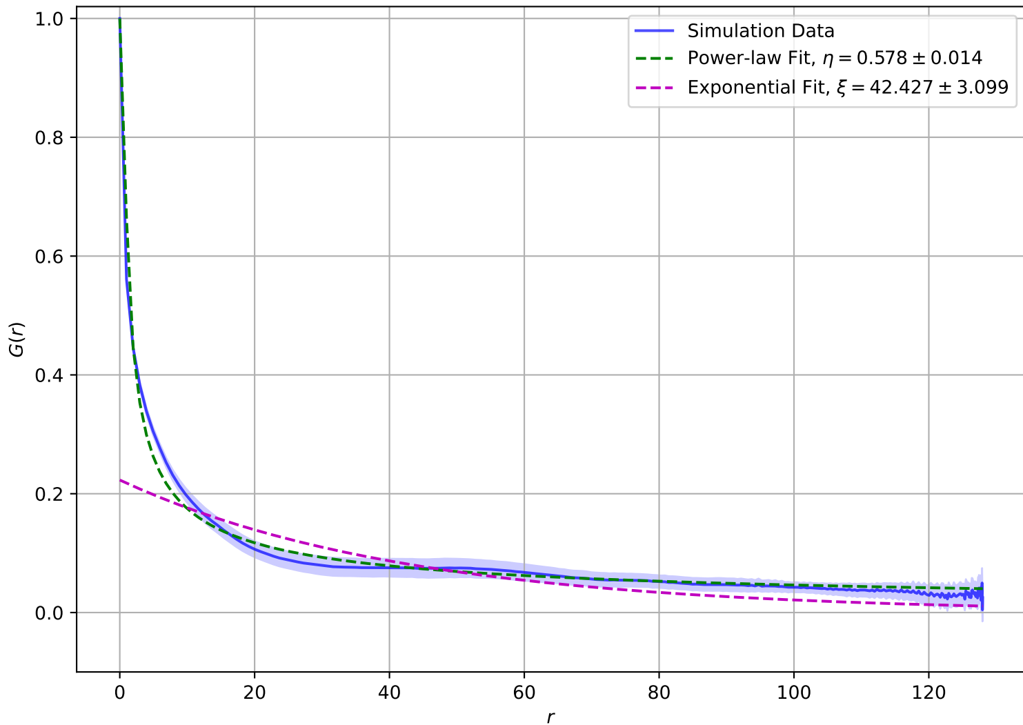
Correlation Function at T = 2.05e - 01 , L = 128
