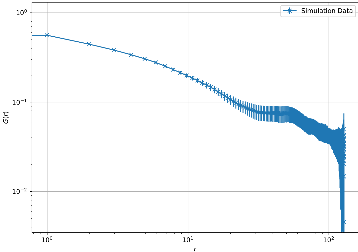
Correlation Function at T = 2.05e - 01 , L = 128 (Log-Log Scale)
