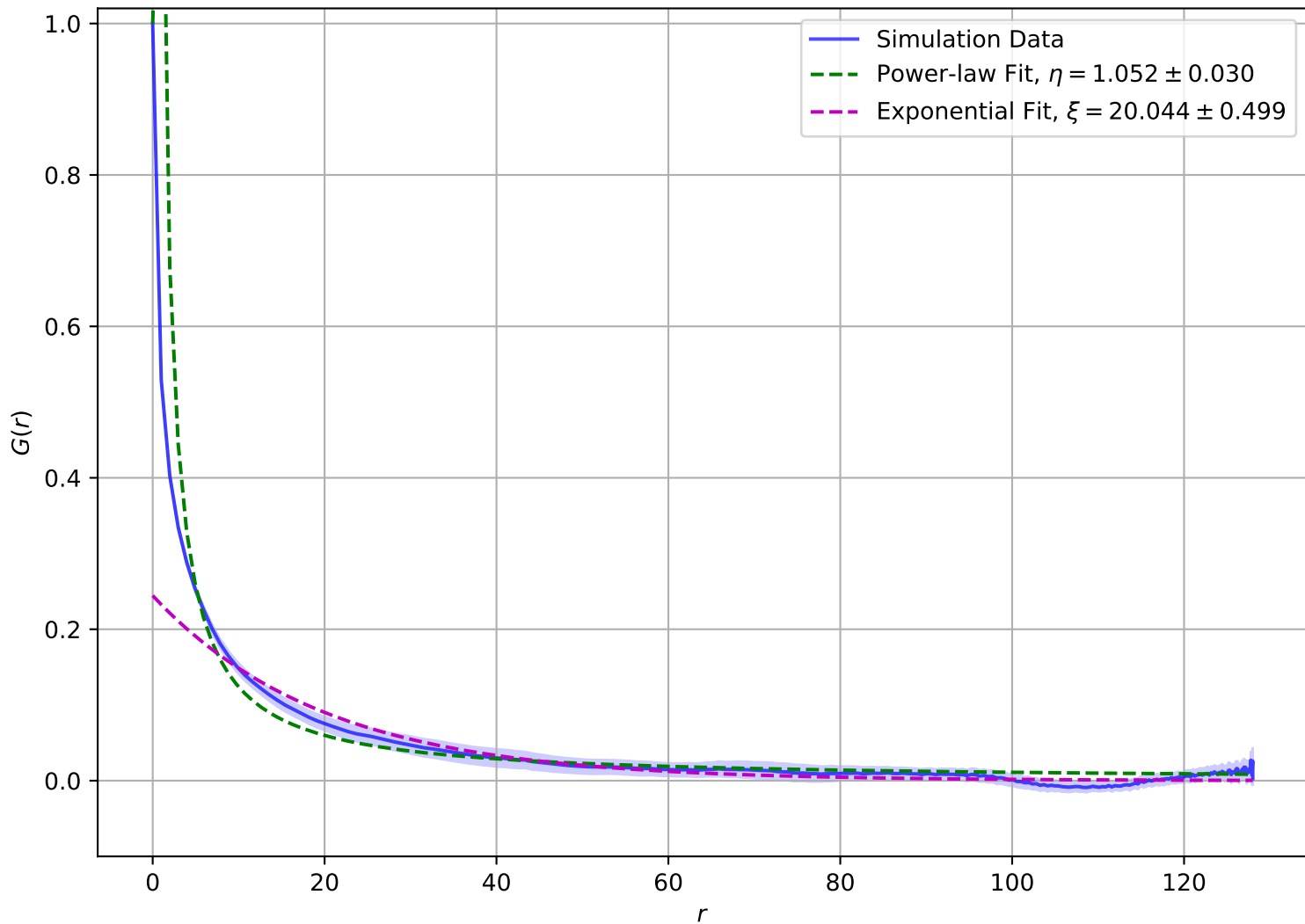
Correlation Function at T = 2.10e - 01 , L = 128
