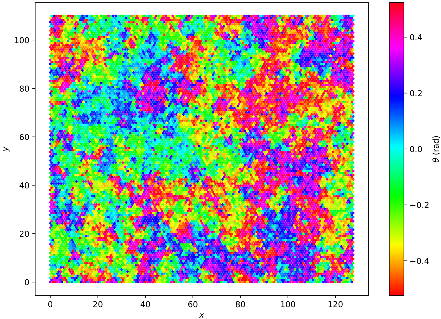
Hexagonal Lattice L=128 , T = 2.10e - 01
