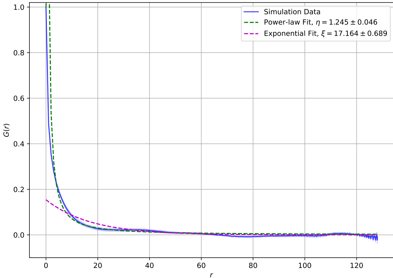
Correlation Function at T = 2.15e - 01 , L = 128
