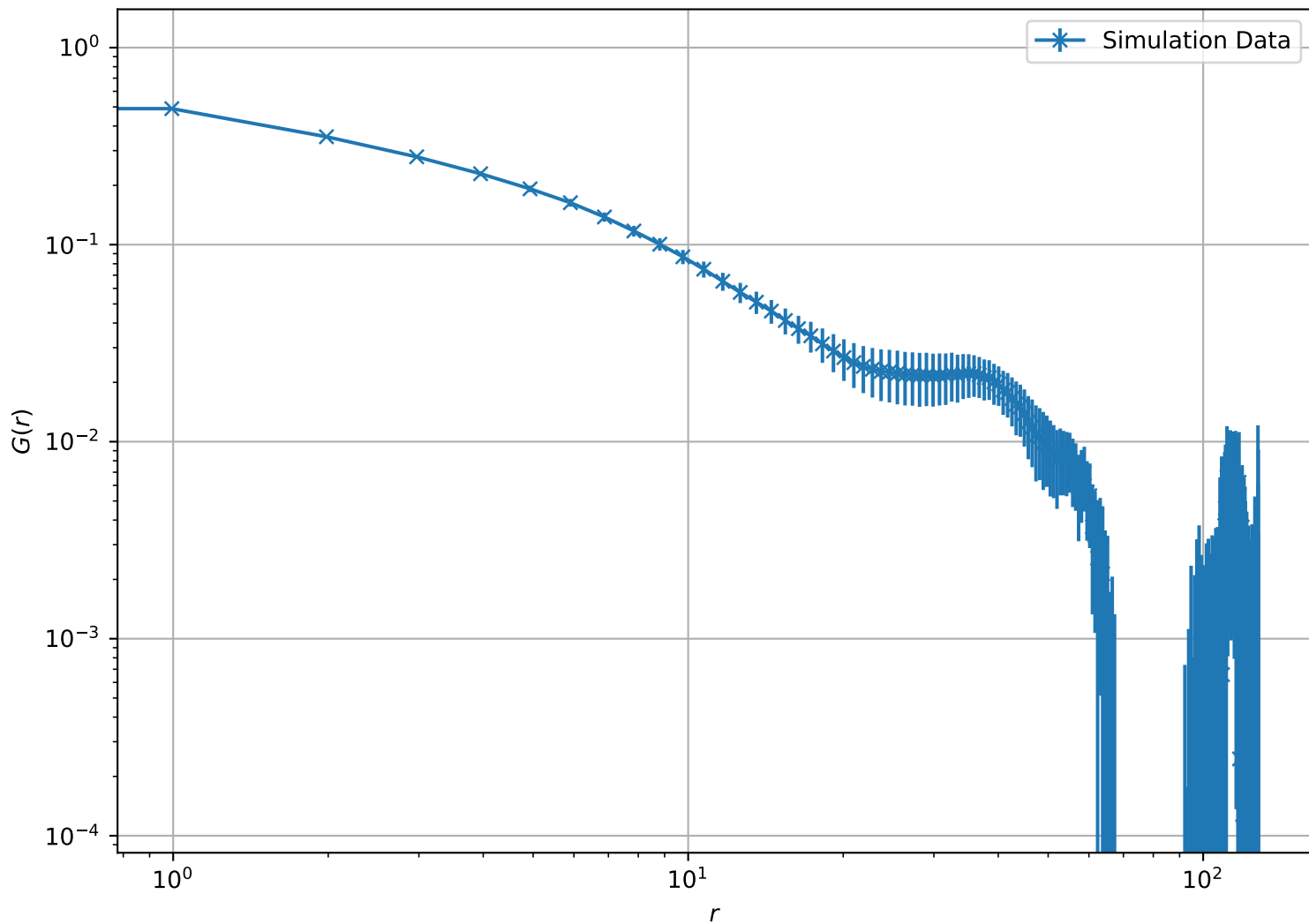
Correlation Function at T = 2.15e - 01 , L = 128 (Log-Log Scale)
