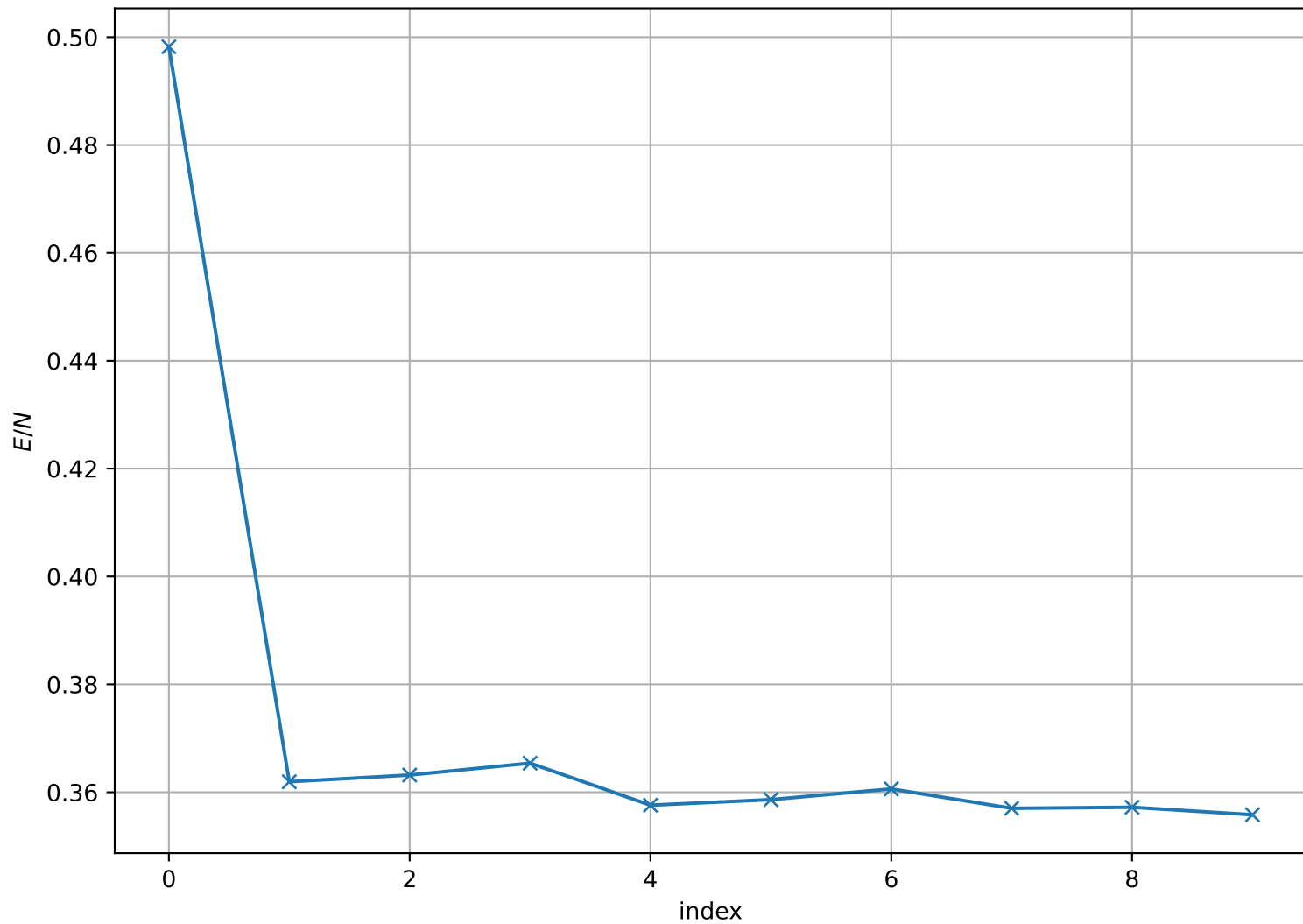
Energy per Site at T = 2.150e - 01 , L = 128
