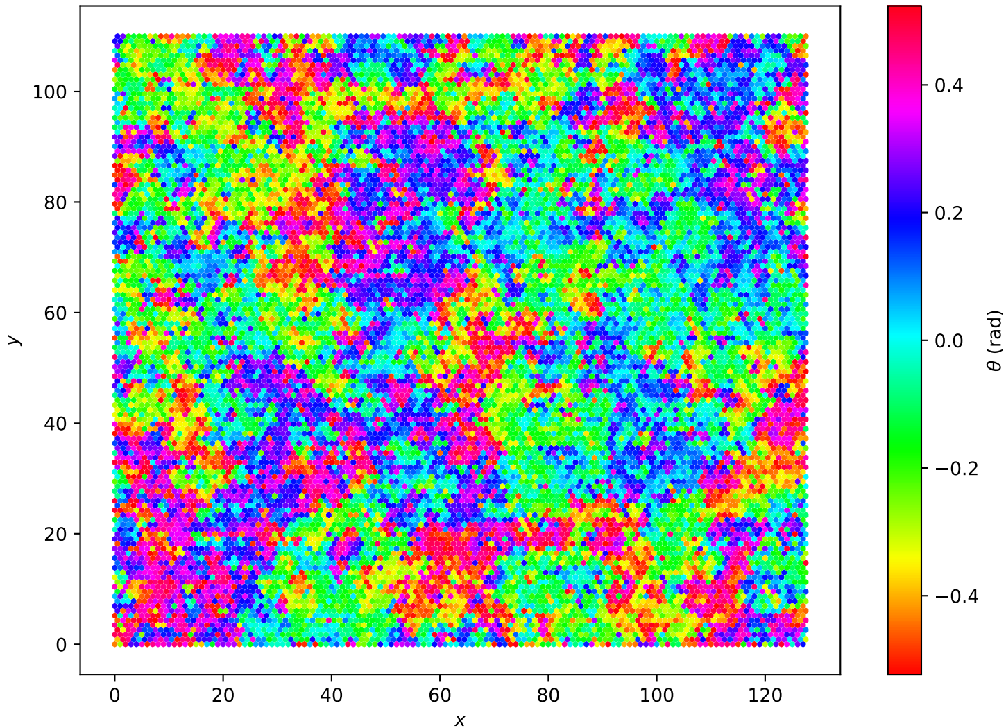
Hexagonal Lattice L=128 , T = 2.15e - 01
