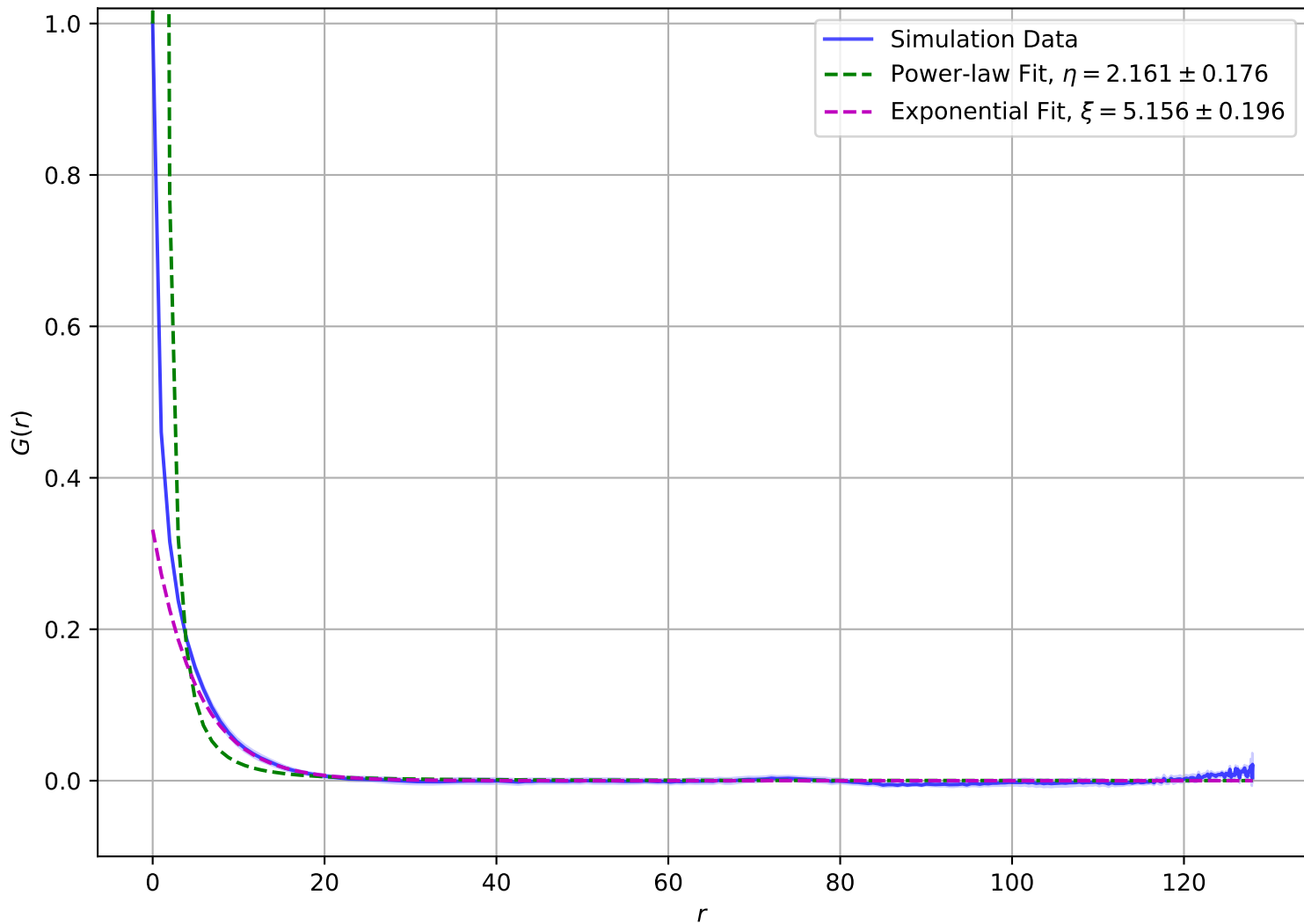
Correlation Function at T = 2.20\text{e} - 01 , L = 128
