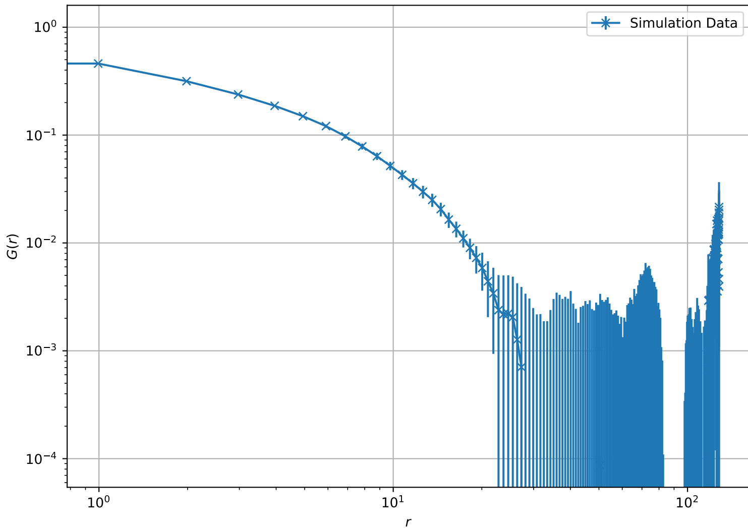
Correlation Function at T = 2.20e - 01 , L = 128 (Log-Log Scale)
