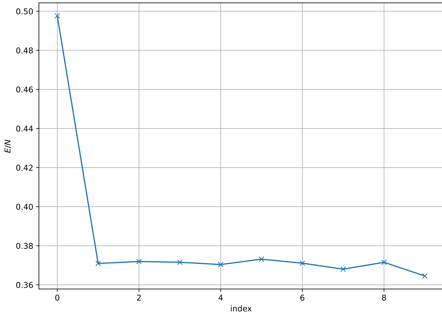
Energy per Site at T = 2.200e - 01 , L = 128
