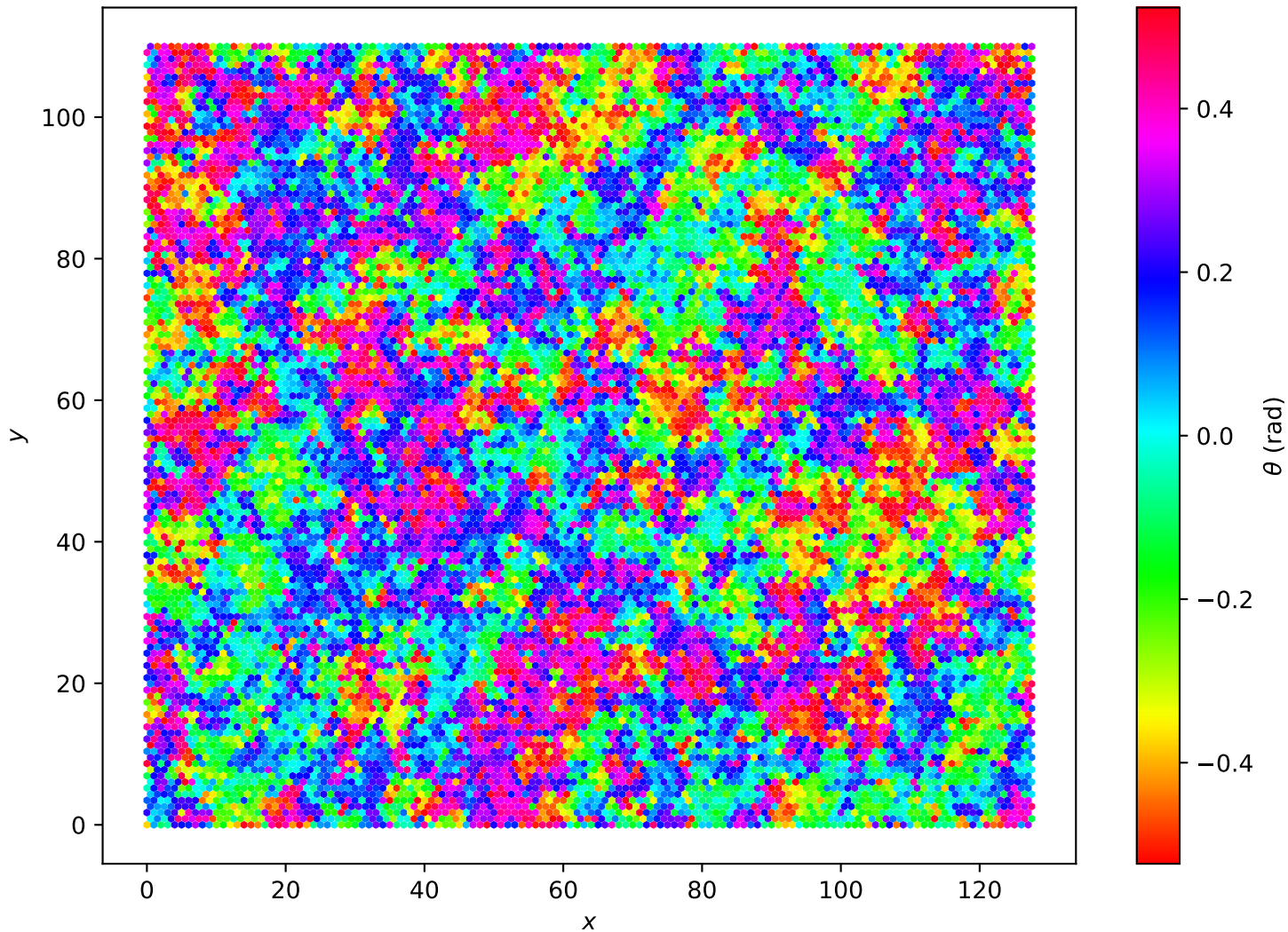
Hexagonal Lattice L=128 , T = 2.20e - 01
