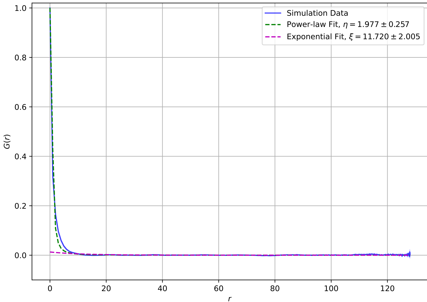
Correlation Function at T = 2.50e - 01 , L = 128
