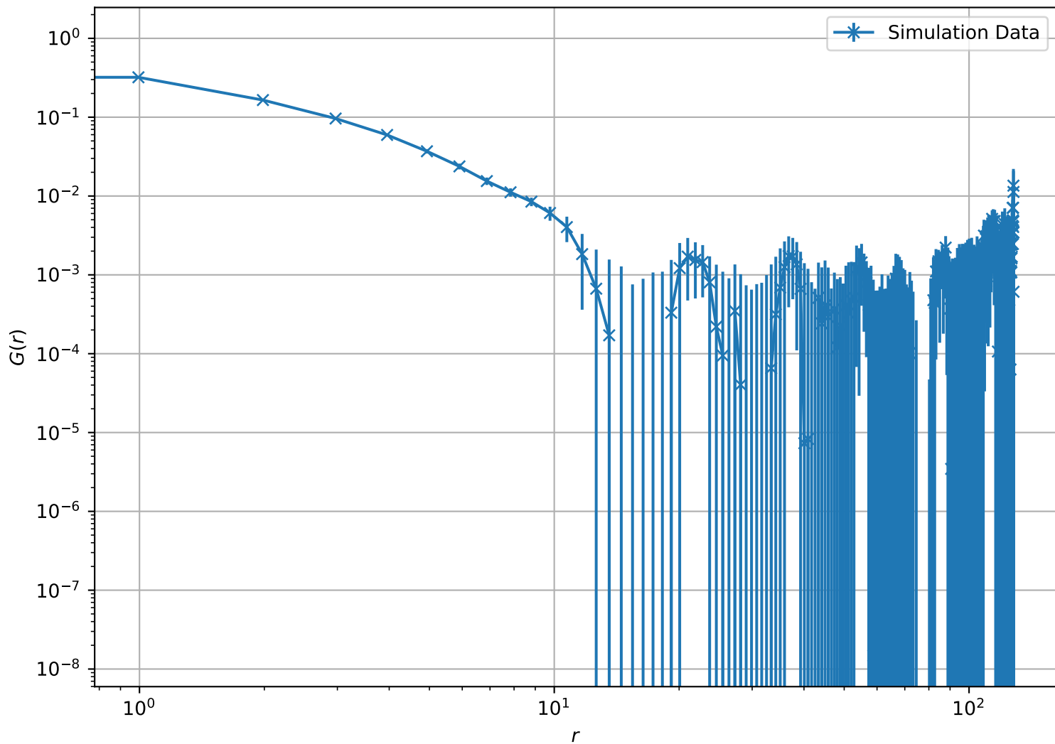
Correlation Function at T = 2.50e - 01 , L = 128 (Log-Log Scale)
