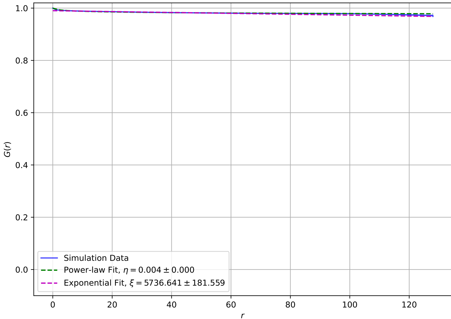
Correlation Function at T = 5.00\text{e} - 02 , L = 128
