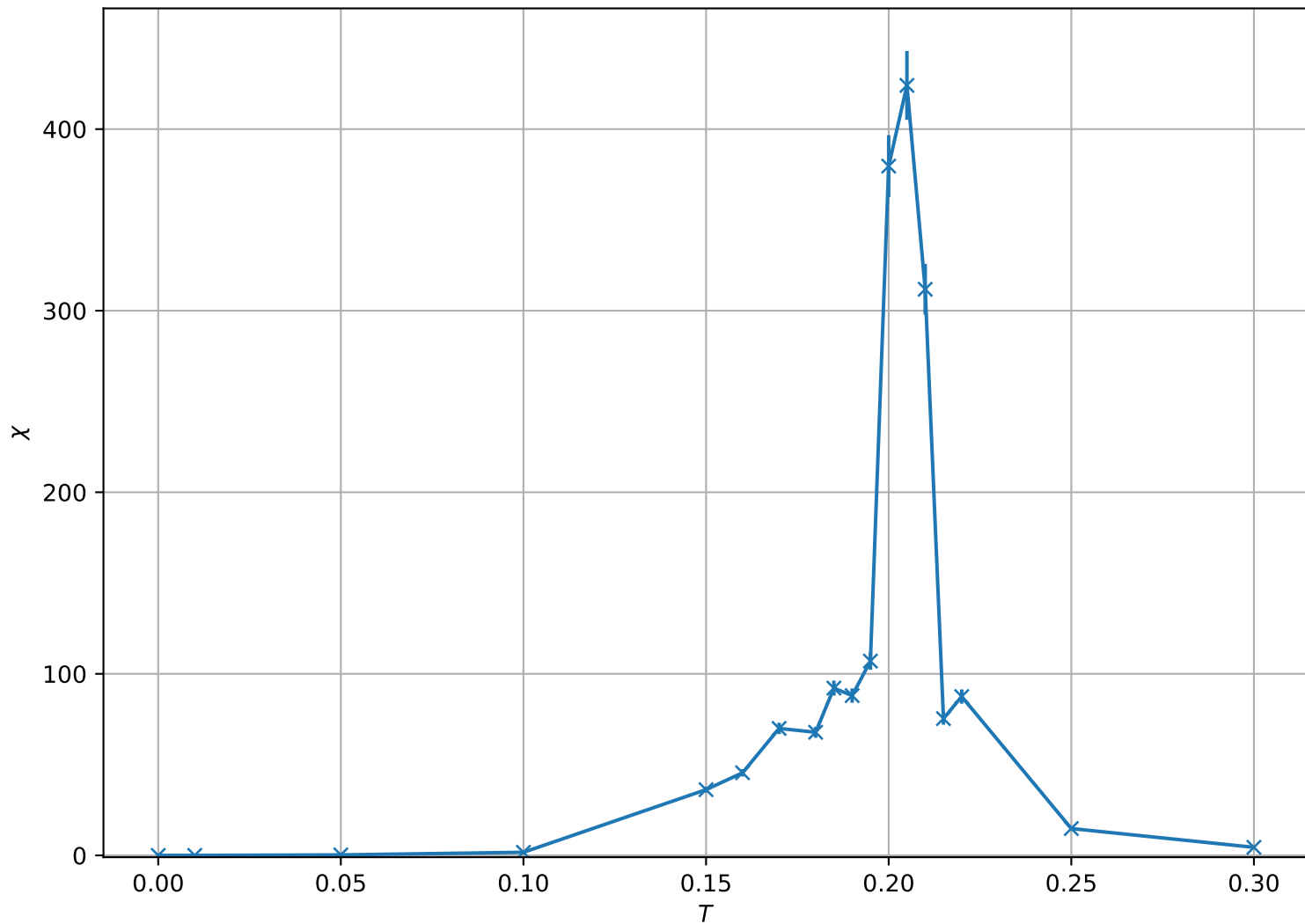
Susceptibility \chi vs Temperature for L = 128
