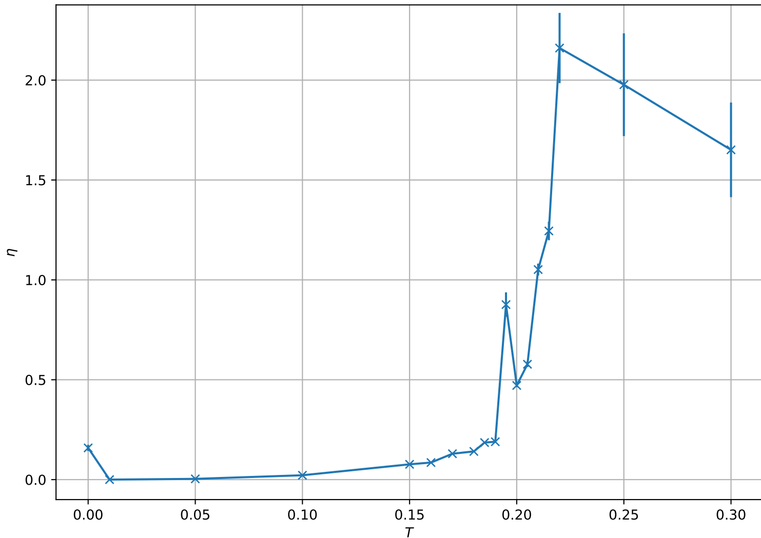
Critical Exponent \eta vs Temperature for L = 128
