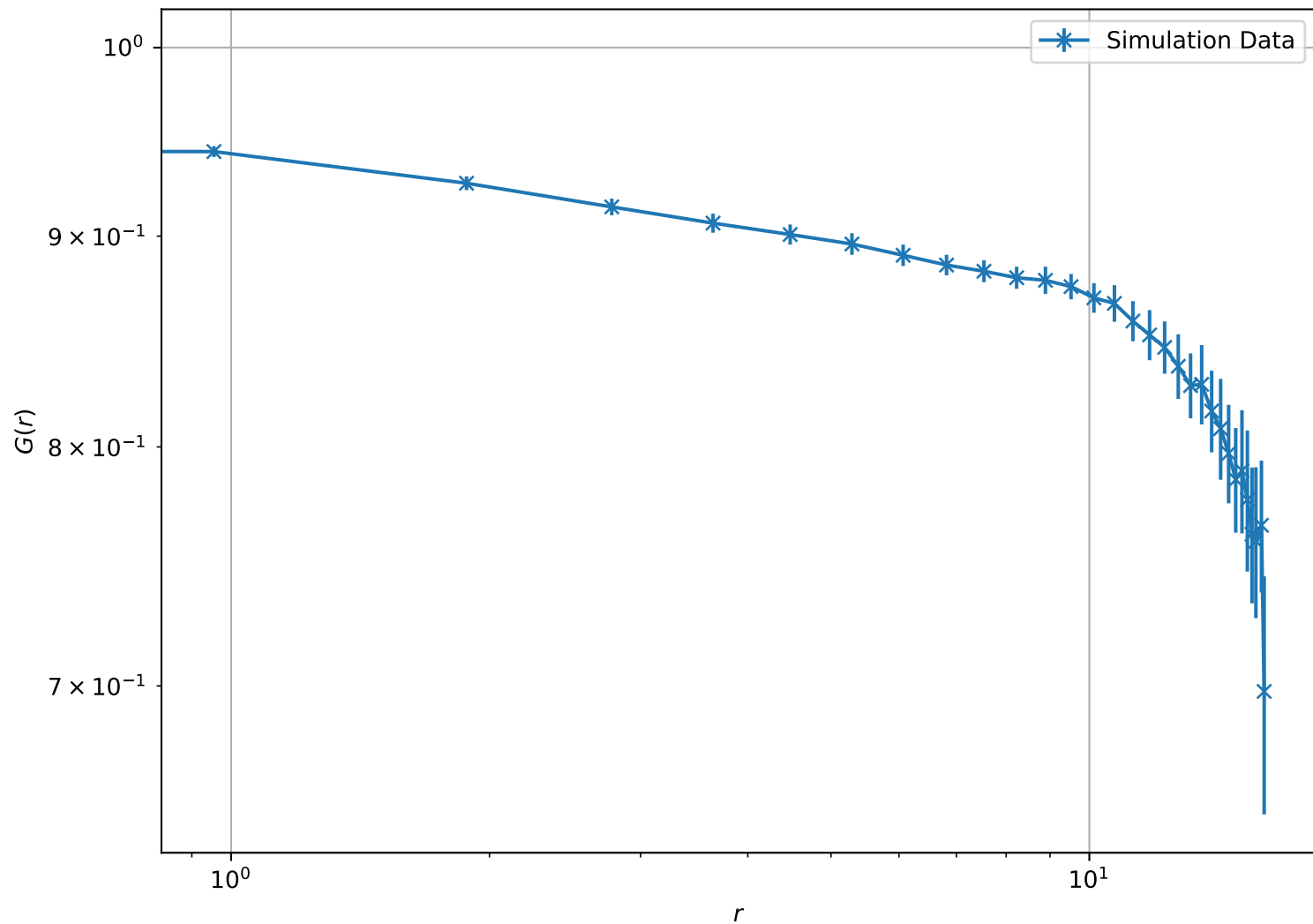
Correlation Function at T = 1.00\text{e} - 01 , L = 16 (Log-Log Scale)
